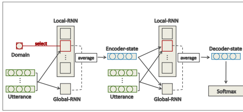
図 1: Local/Global SEQ2SEQ
