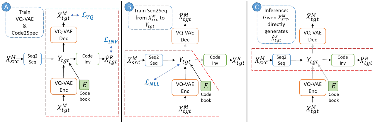
Figure 1: a) Train VQ-VAE to represent continuous MFCC vectors with codebook sequence and train codebook inverter to generate a linear magnitude spectrogram based on generated codebook sequence; b) Train a seq2seq model from source language MFCC to target language codebook. c) In inference stage, seq2seq model takes source language MFCC and predicts codebook sequences, and then codebook inverter generates target language speech representation.
